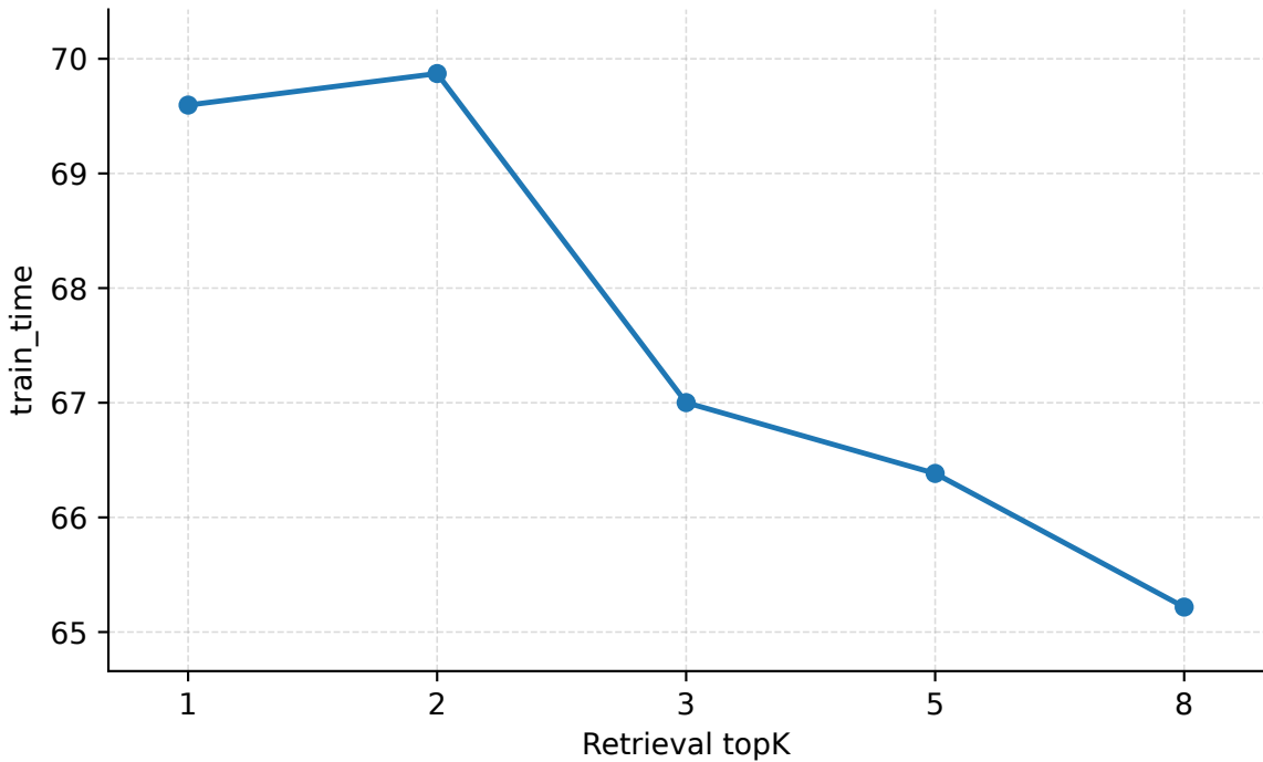
Retrieval topK | Geant | PredLen=5 | train_time
