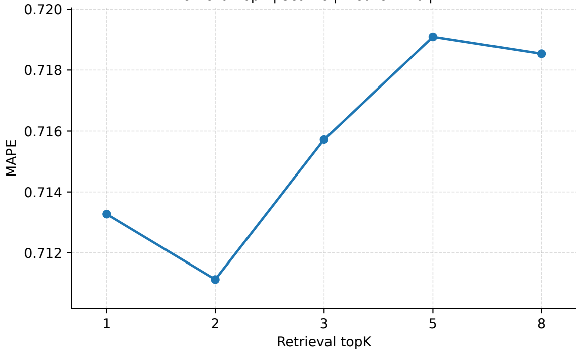
Retrieval topK | Seattle | PredLen=10 | MAPE
