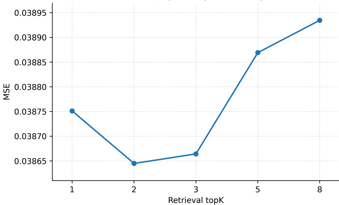
Retrieval topK | Seattle | PredLen=10 | MSE
