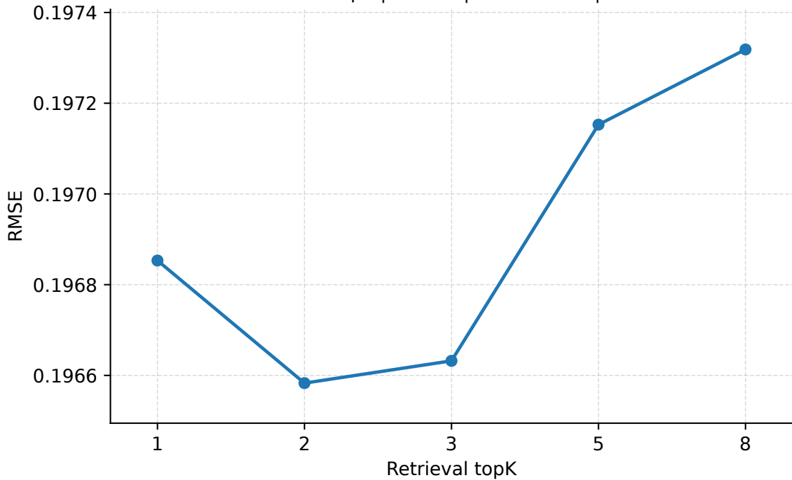
Retrieval topK | Seattle | PredLen=10 | RMSE
