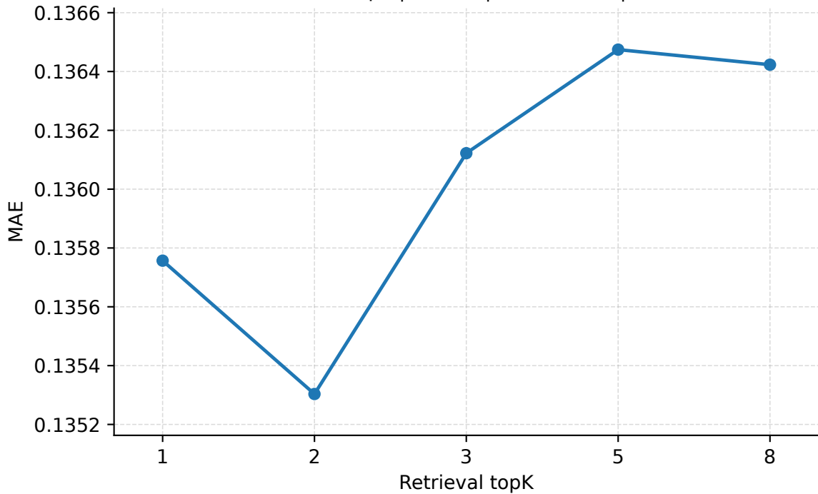
Retrieval topK | Seattle | PredLen=15 | MAE
