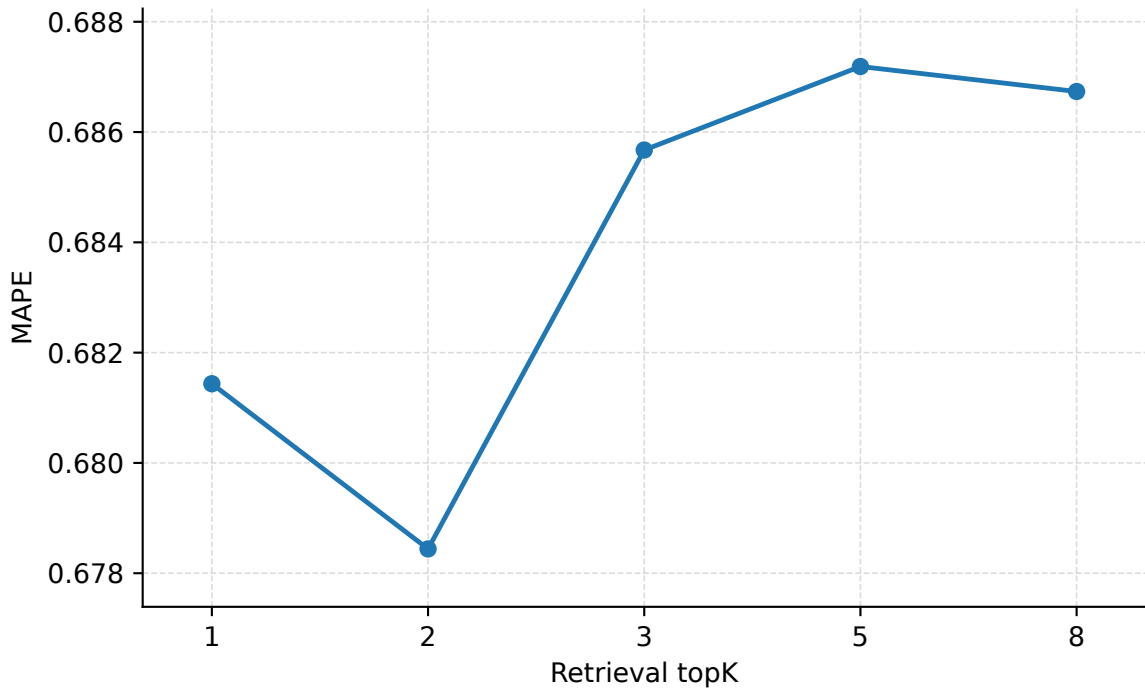
Retrieval topK | Seattle | PredLen=15 | MAPE
