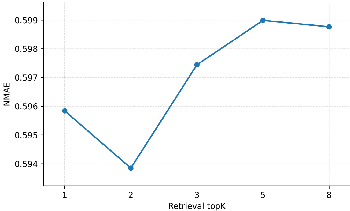
Retrieval topK | Seattle | PredLen=15 | NMAE
