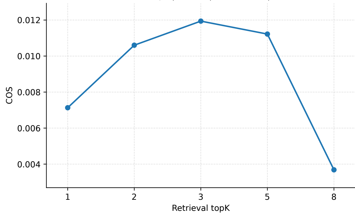
Retrieval topK | Seattle | PredLen=20 | COS
