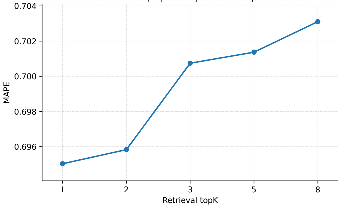
Retrieval topK | Seattle | PredLen=20 | MAPE
