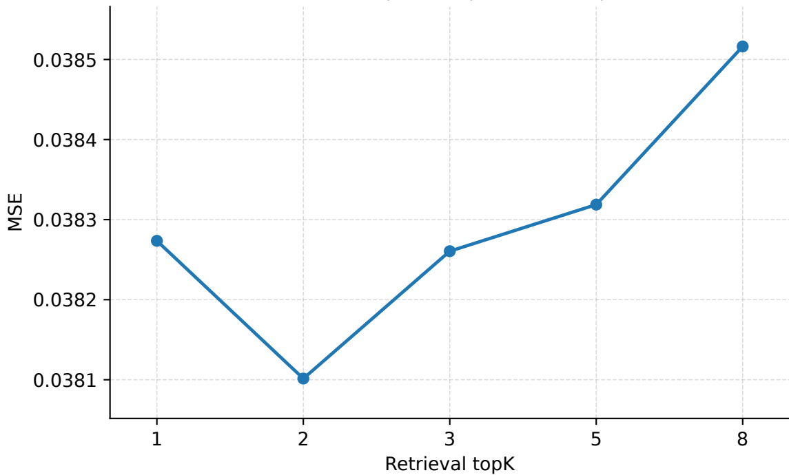
Retrieval topK | Seattle | PredLen=20 | MSE
