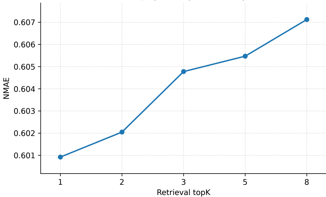
Retrieval topK | Seattle | PredLen=20 | NMAE
