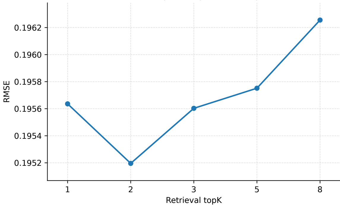
Retrieval topK | Seattle | PredLen=20 | RMSE
