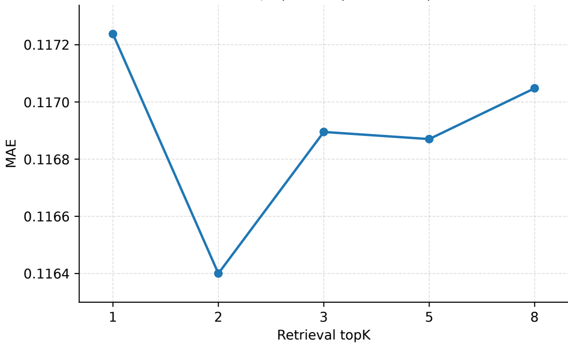
Retrieval topK | Seattle | PredLen=5 | MAE
