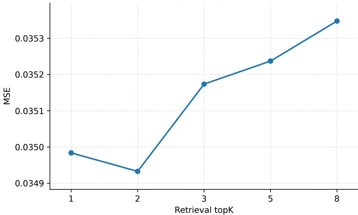
Retrieval topK | Seattle | PredLen=5 | MSE
