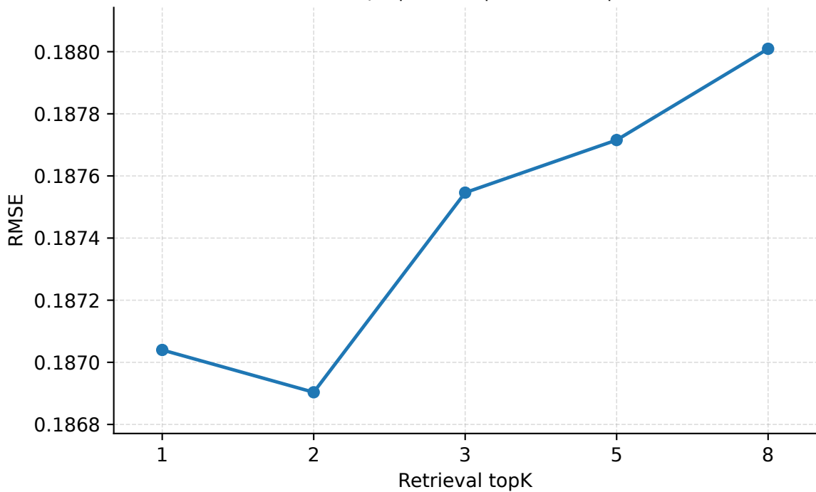
Retrieval topK | Seattle | PredLen=5 | RMSE
