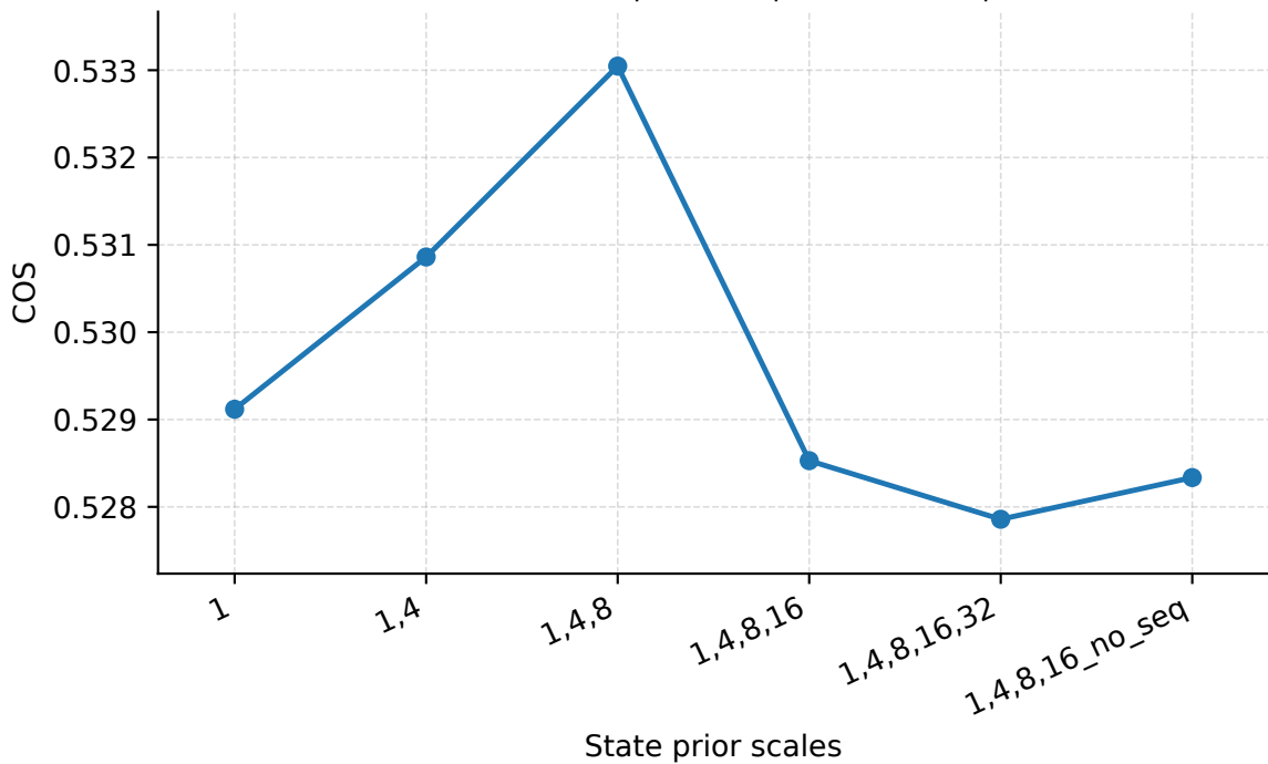
State Prior Scales | Abilene | PredLen=10 | COS
