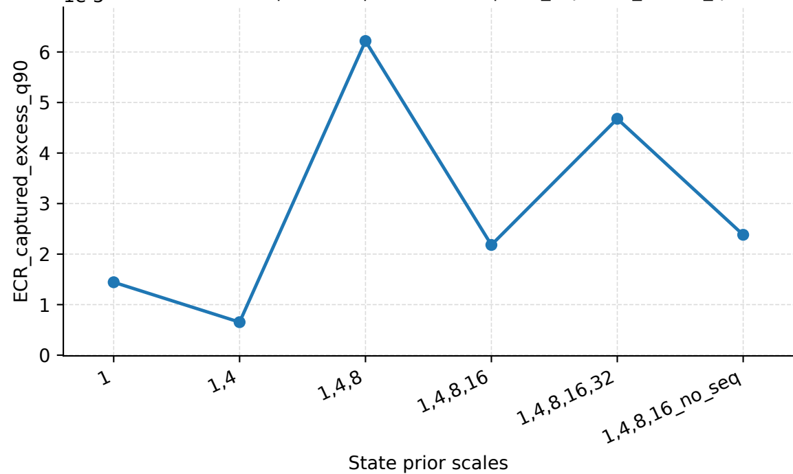
1e-5 State Prior Scales | Abilene | PredLen=10 | ECR_captured_excess_q90
