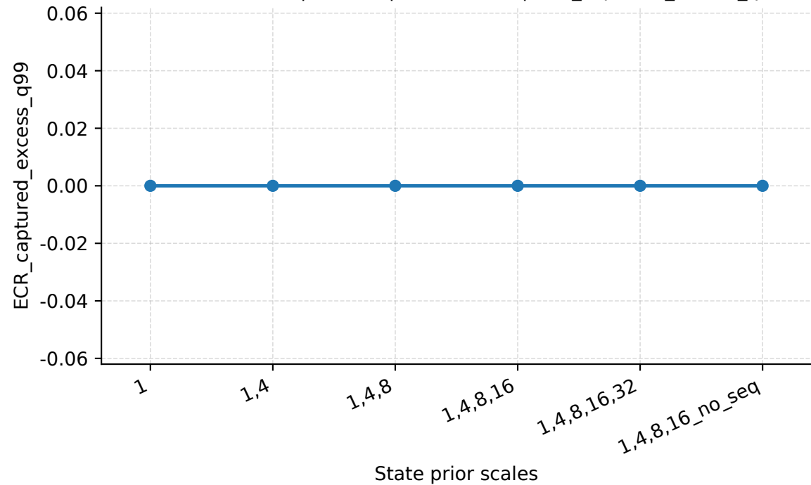
State Prior Scales | Abilene | PredLen=10 | ECR_captured_excess_q99
