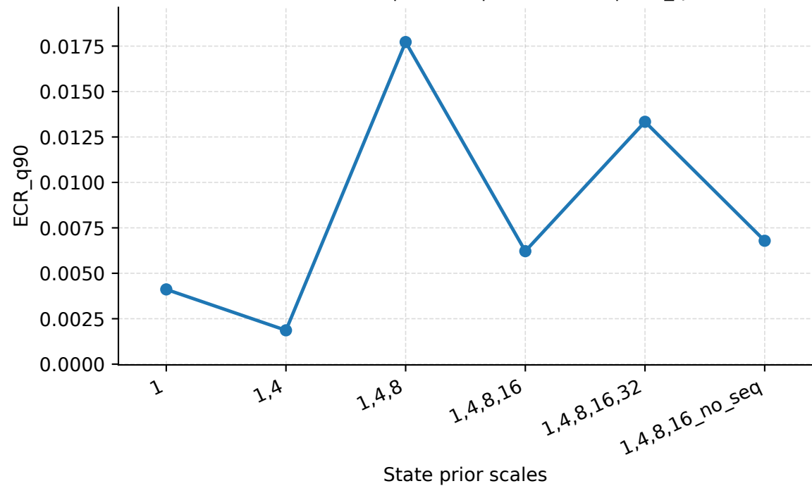
State Prior Scales | Abilene | PredLen=10 | ECR_q90
