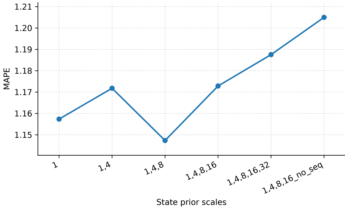
State Prior Scales | Abilene | PredLen=10 | MAPE
