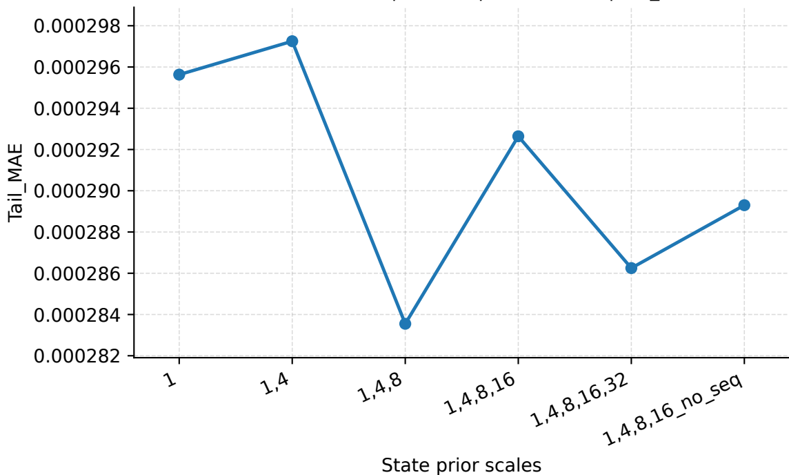
State Prior Scales | Abilene | PredLen=10 | Tail_MAE
