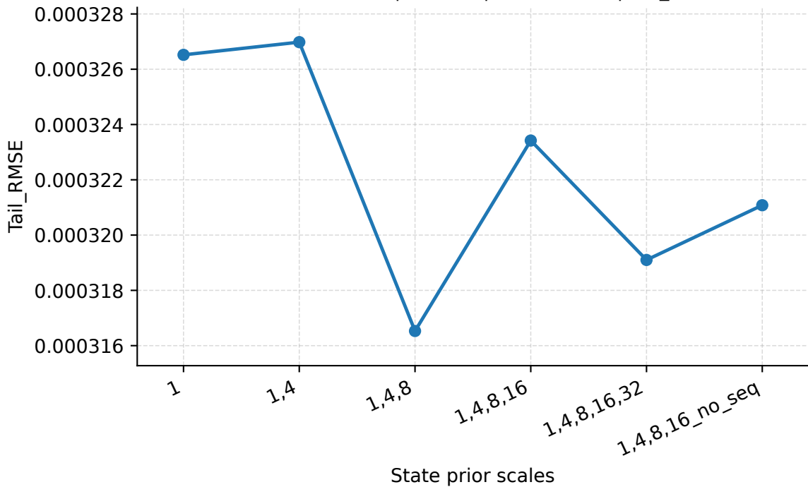
State Prior Scales | Abilene | PredLen=10 | Tail_RMSE
