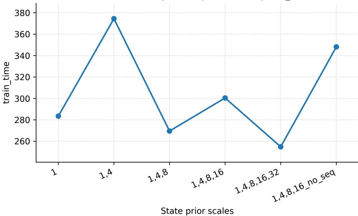
State Prior Scales | Abilene | PredLen=10 | train_time
