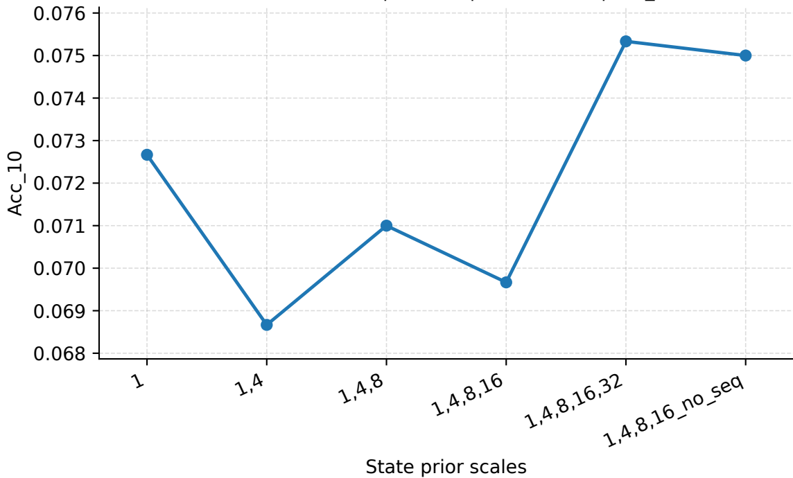
State Prior Scales | Abilene | PredLen=15 | Acc_10
