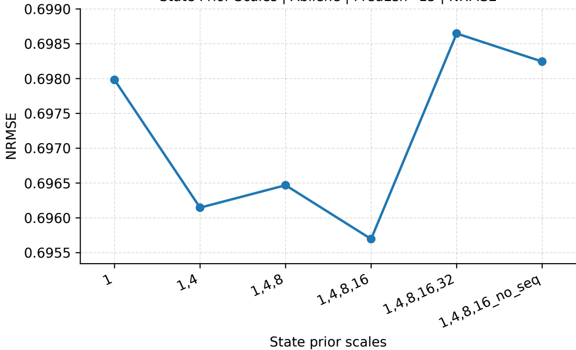
State Prior Scales | Abilene | PredLen=15 | NRMSE
