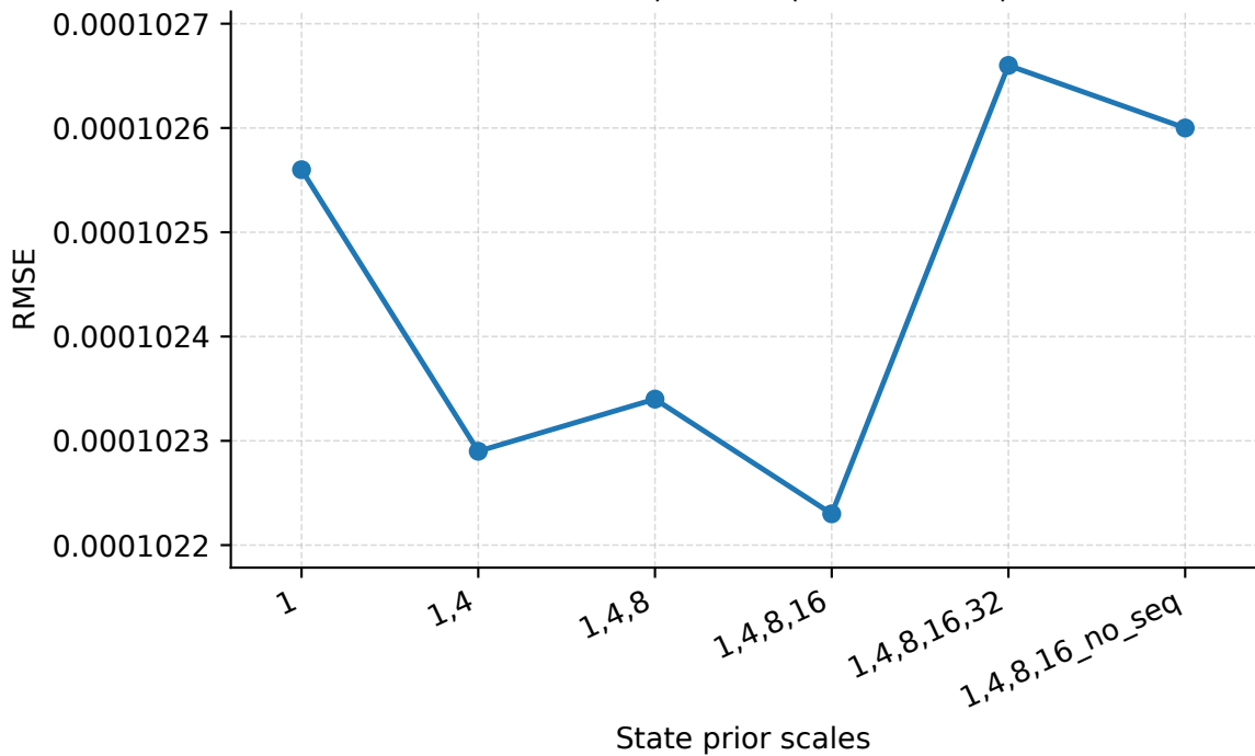
State Prior Scales | Abilene | PredLen=15 | RMSE
