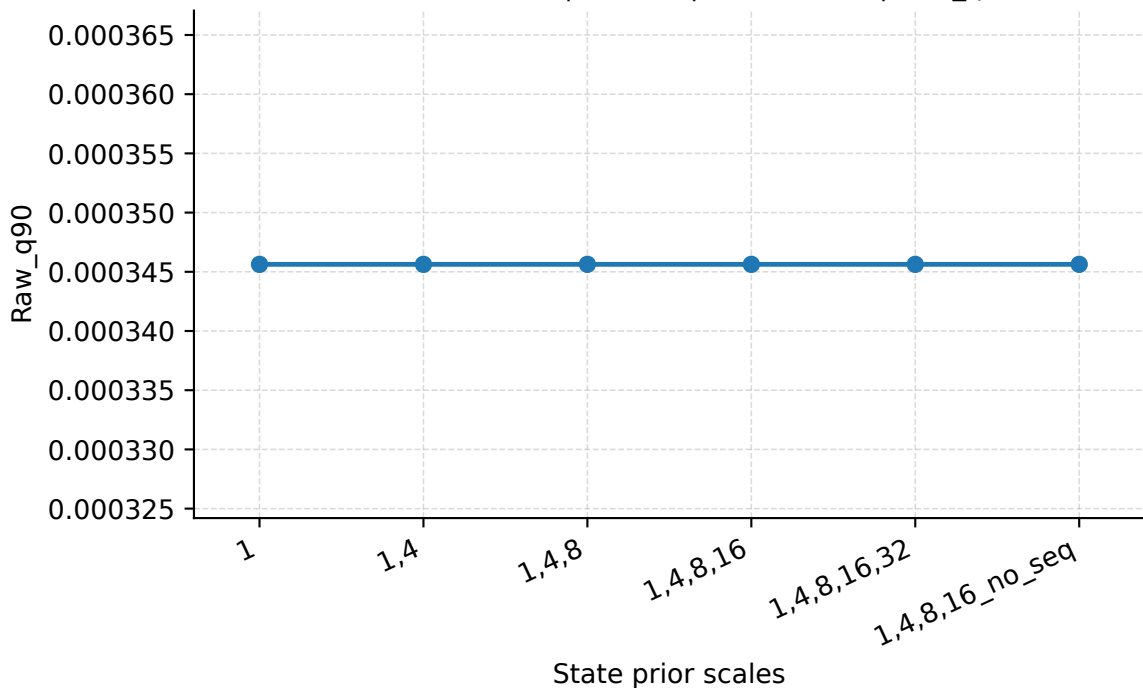
State Prior Scales | Abilene | PredLen=15 | Raw_q90
