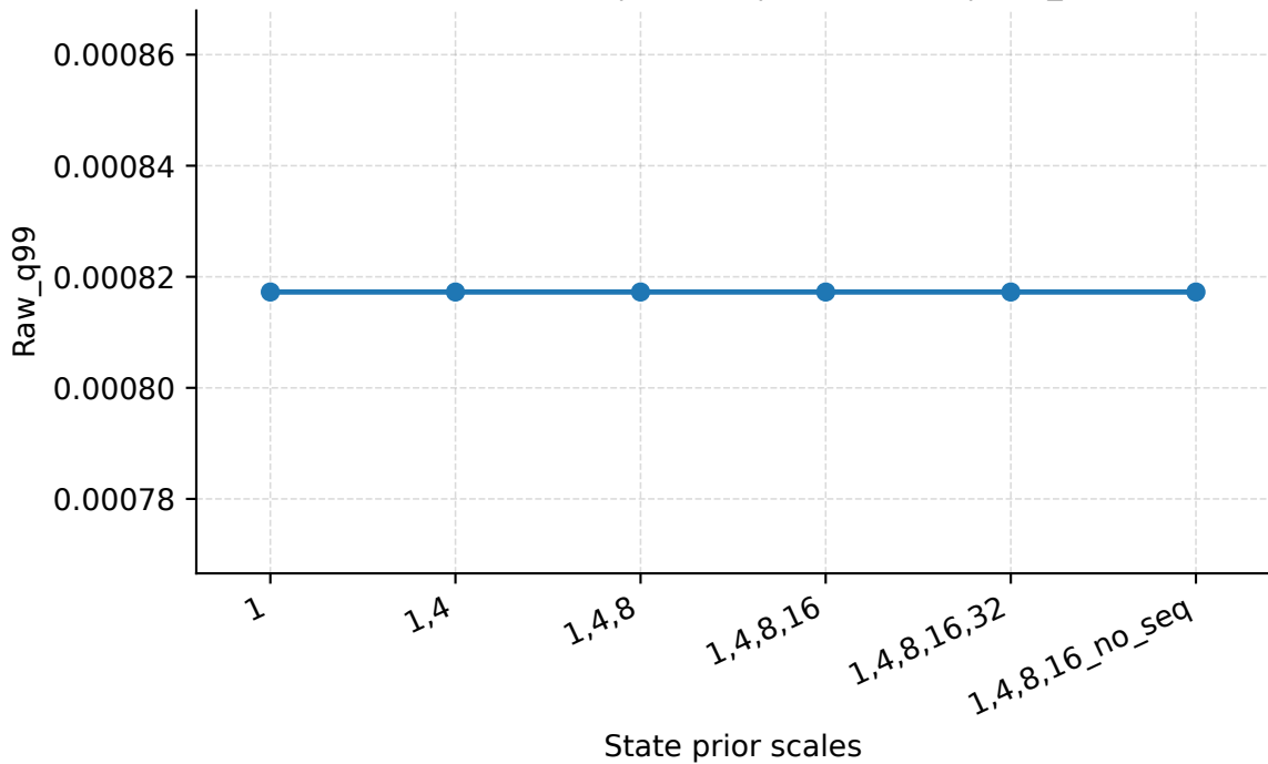
State Prior Scales | Abilene | PredLen=15 | Raw_q99
