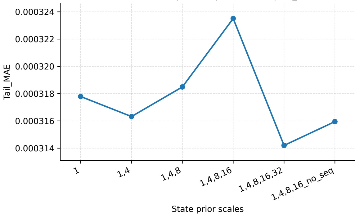
State Prior Scales | Abilene | PredLen=15 | Tail_MAE
