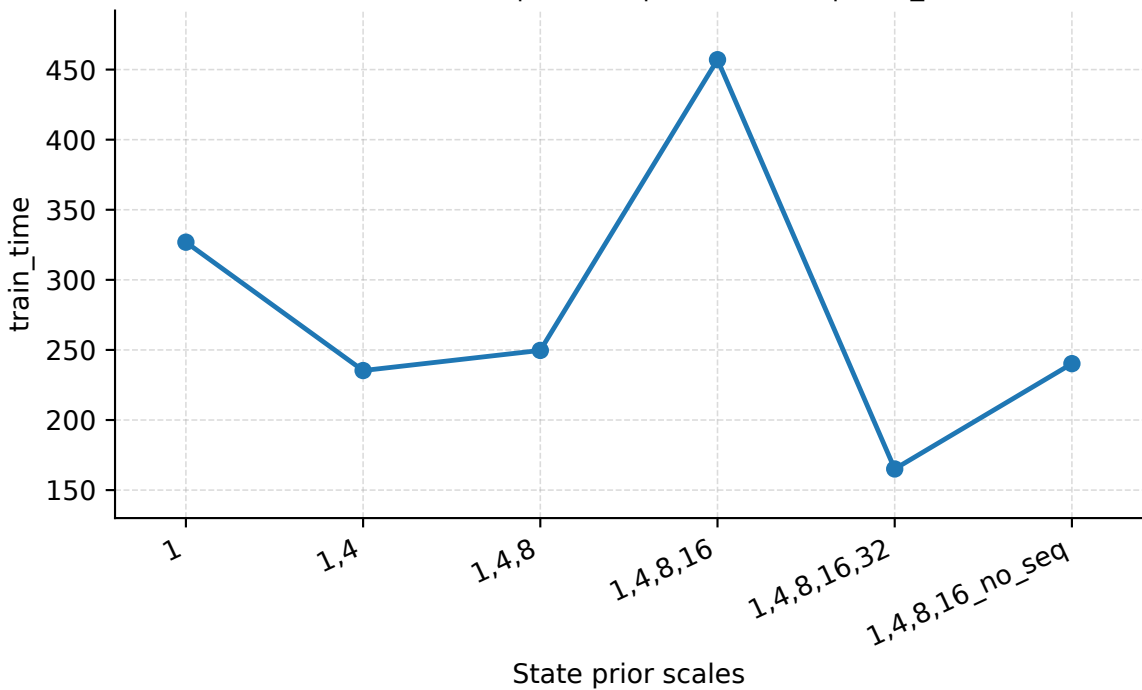
State Prior Scales | Abilene | PredLen=15 | train_time
