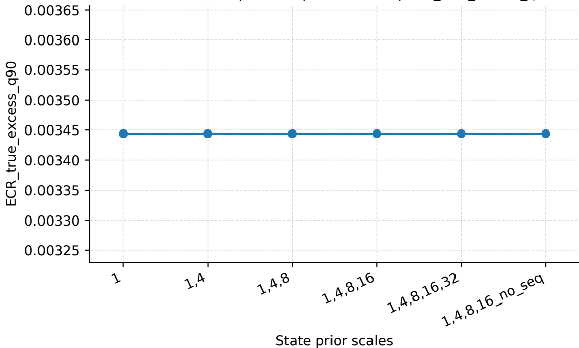
State Prior Scales | Abilene | PredLen=20 | ECR_true_excess_q90
