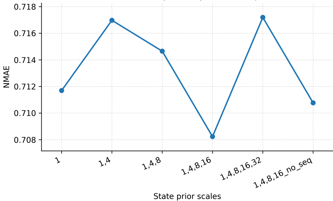
State Prior Scales | Abilene | PredLen=20 | NMAE
