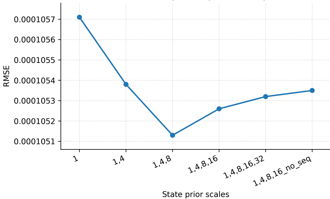
State Prior Scales | Abilene | PredLen=20 | RMSE
