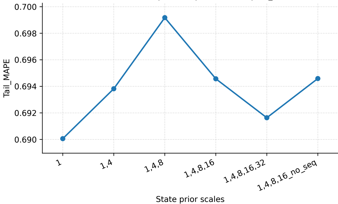
State Prior Scales | Abilene | PredLen=20 | Tail_MAPE
