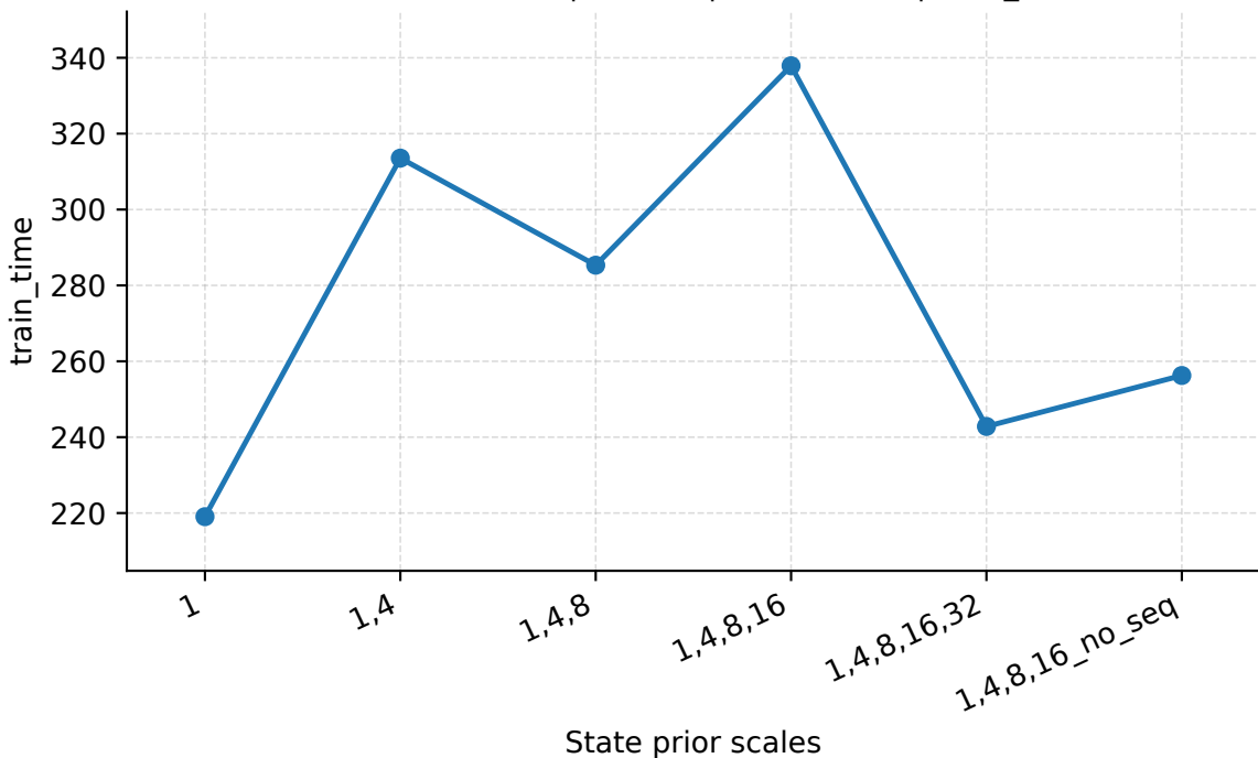
State Prior Scales | Abilene | PredLen=20 | train_time
