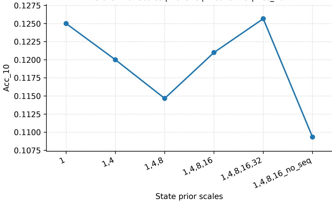
State Prior Scales | Abilene | PredLen=5 | Acc_10
