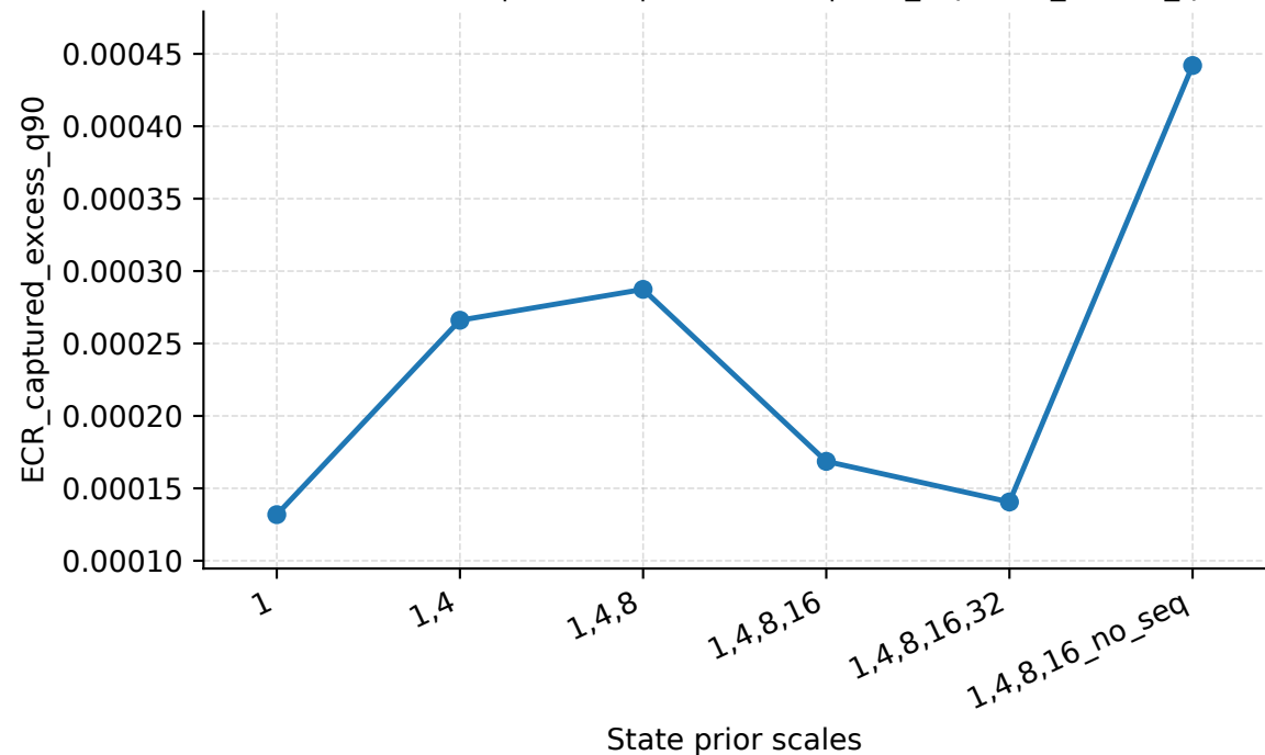
State Prior Scales | Abilene | PredLen=5 | ECR_captured_excess_q90
