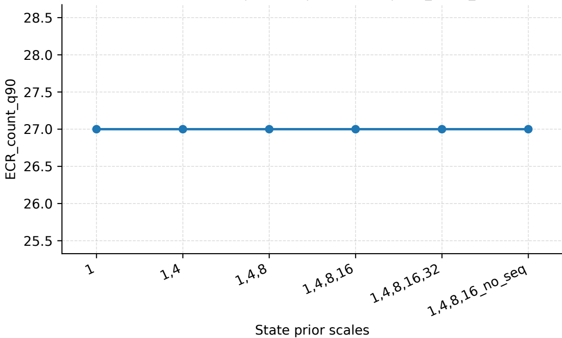
State Prior Scales | Abilene | PredLen=5 | ECR_count_q90
