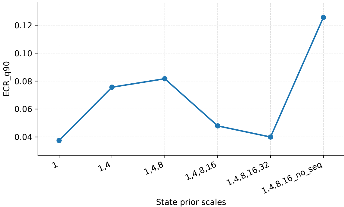
State Prior Scales | Abilene | PredLen=5 | ECR_q90
