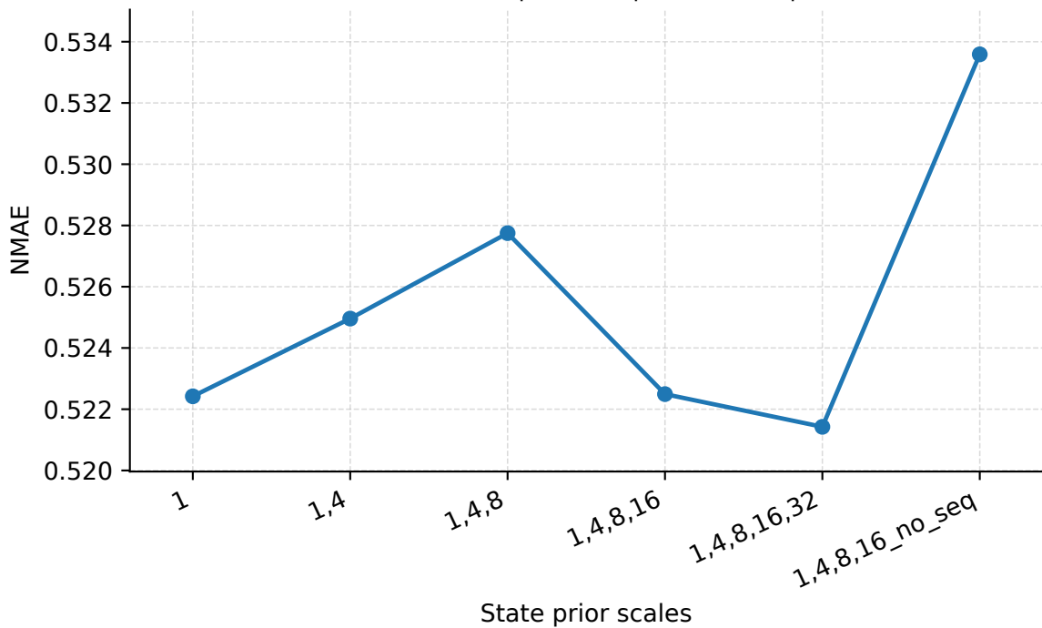
State Prior Scales | Abilene | PredLen=5 | NMAE
