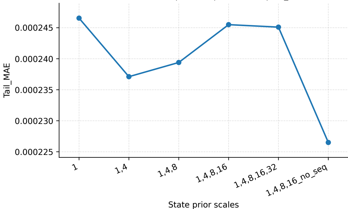
State Prior Scales | Abilene | PredLen=5 | Tail_MAE
