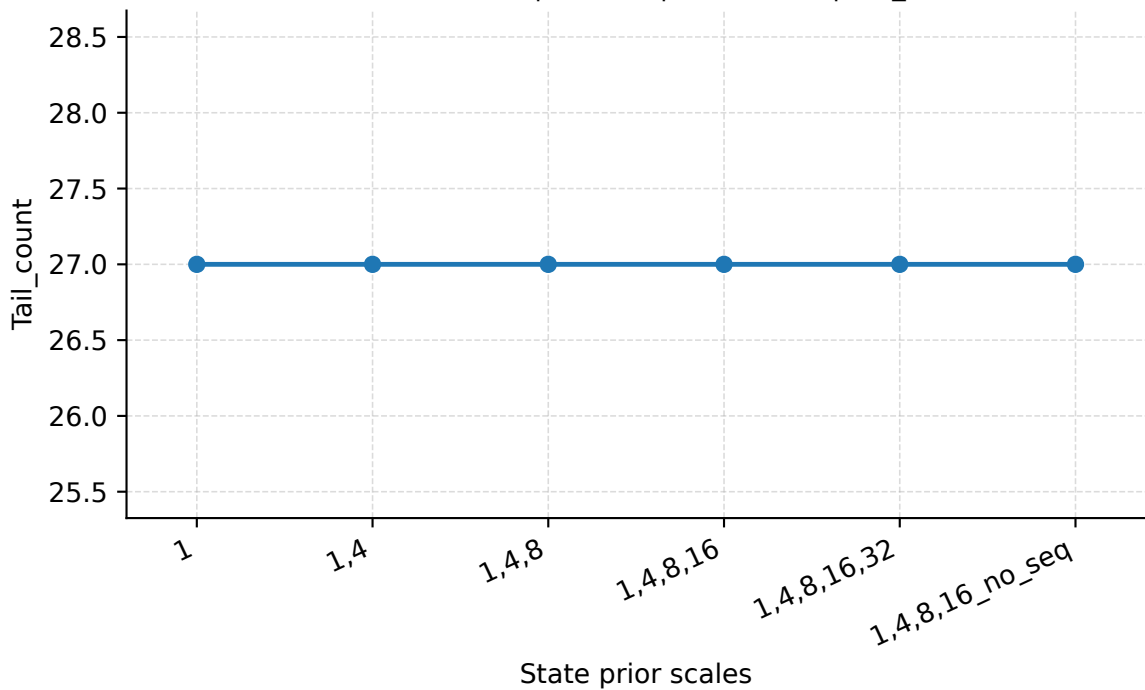
State Prior Scales | Abilene | PredLen=5 | Tail_count
