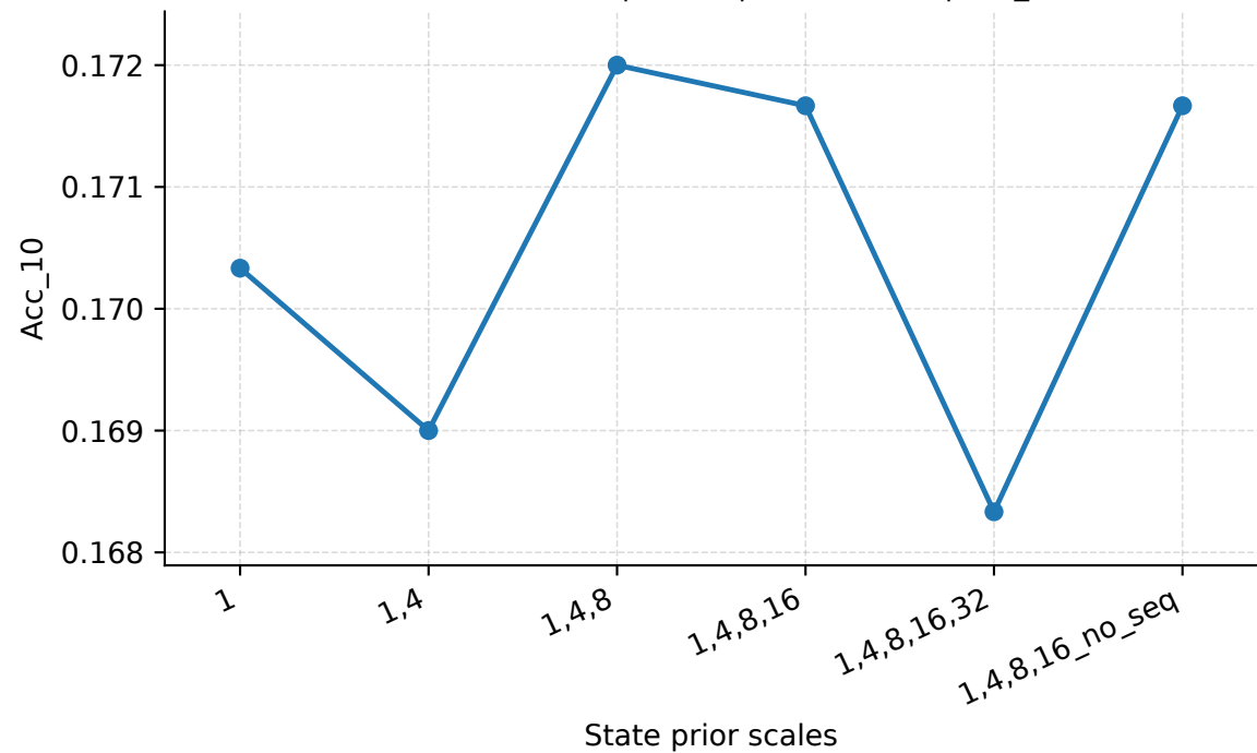
State Prior Scales | Geant | PredLen=10 | Acc_10
