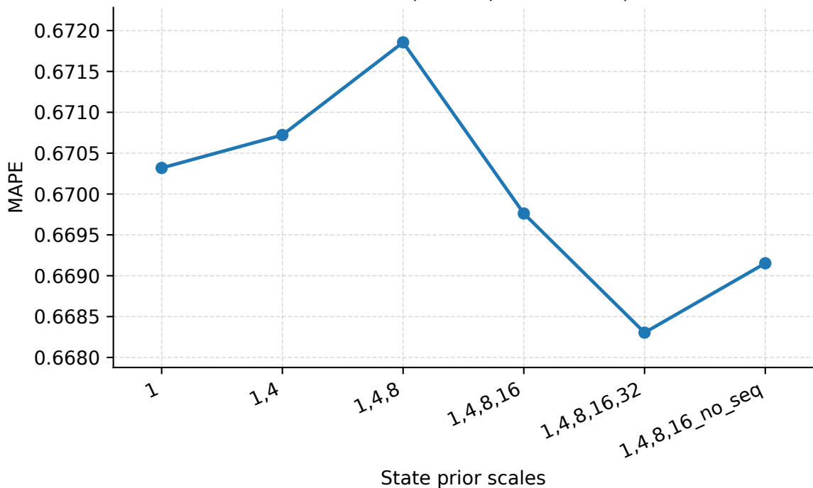
State Prior Scales | Geant | PredLen=10 | MAPE
