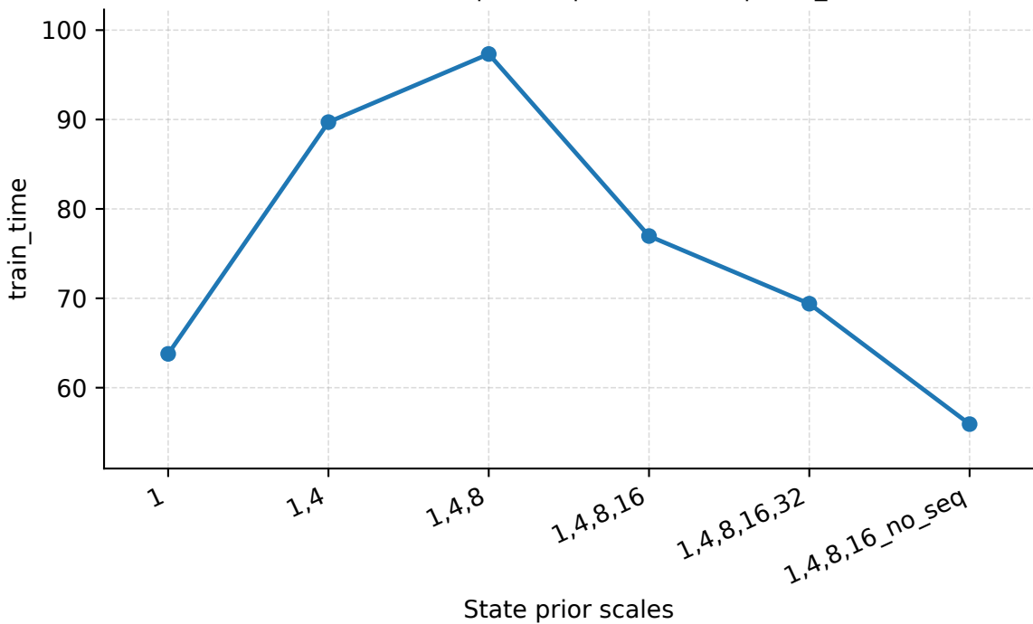
State Prior Scales | Geant | PredLen=10 | train_time
