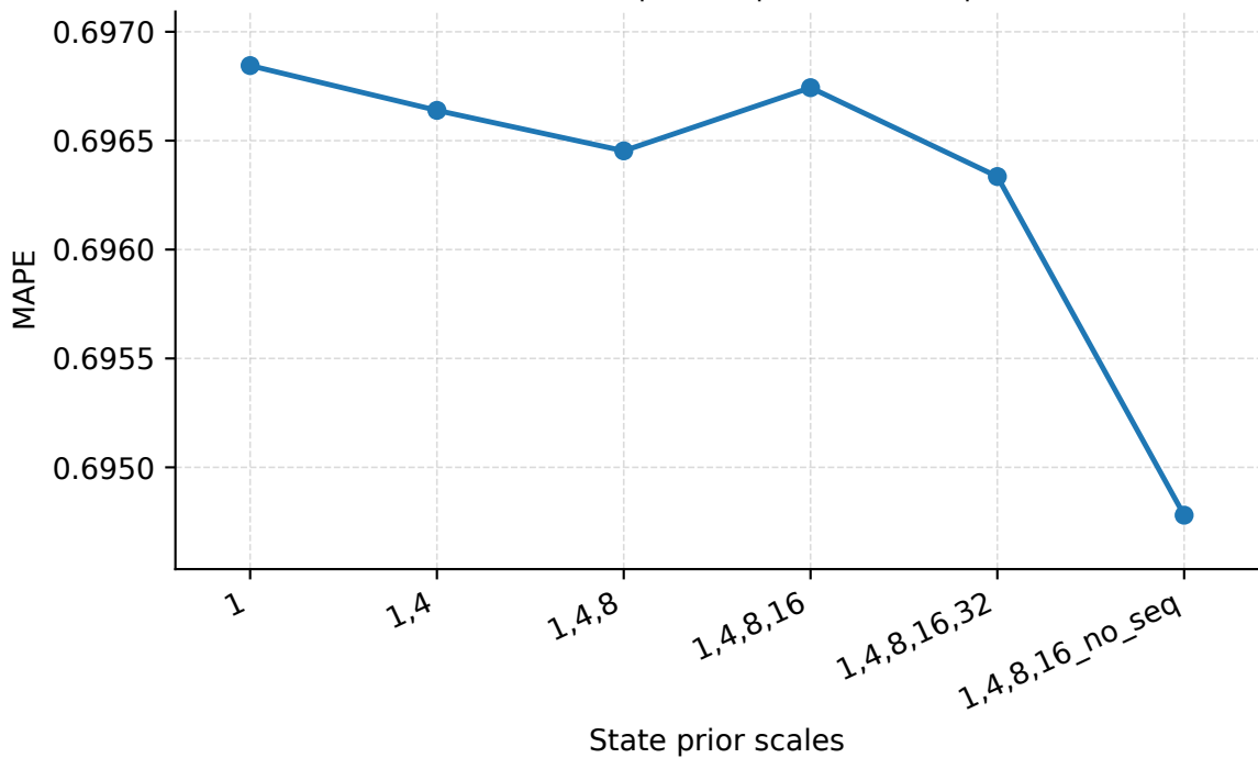
State Prior Scales | Geant | PredLen=15 | MAPE
