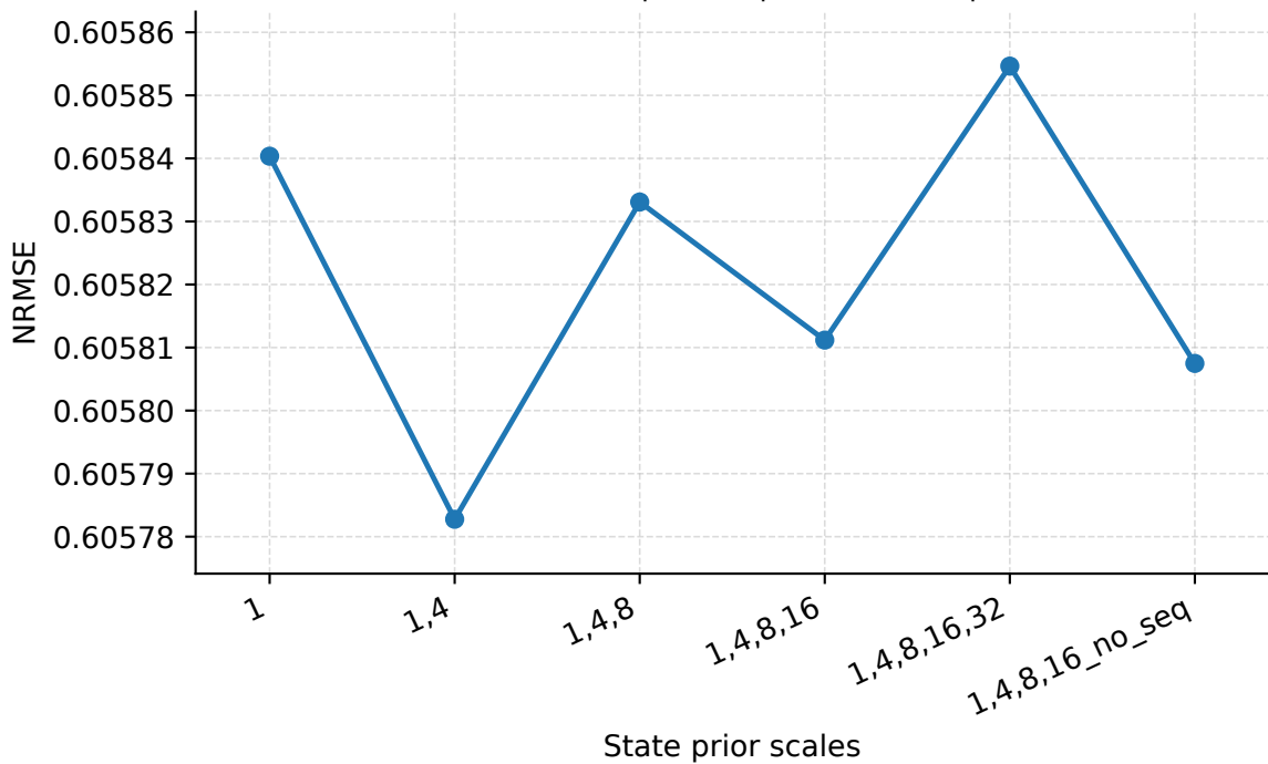
State Prior Scales | Geant | PredLen=15 | NRMSE
