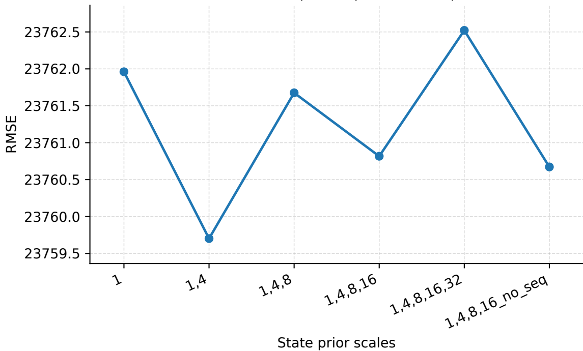
State Prior Scales | Geant | PredLen=15 | RMSE
