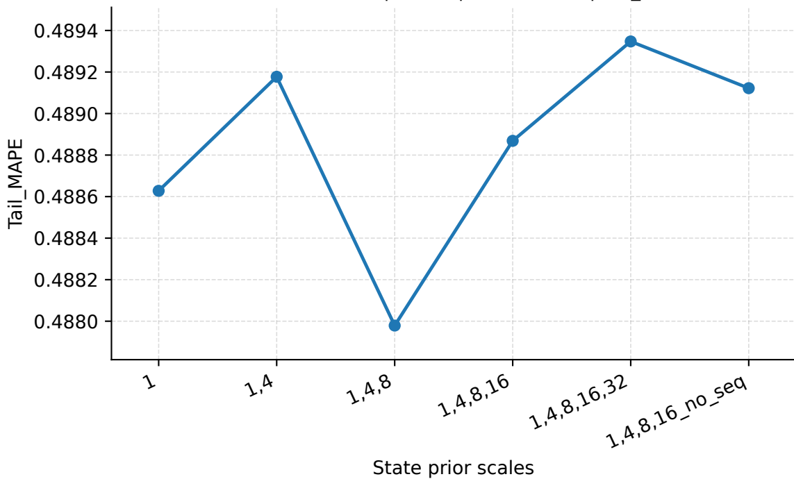
State Prior Scales | Geant | PredLen=15 | Tail_MAPE
