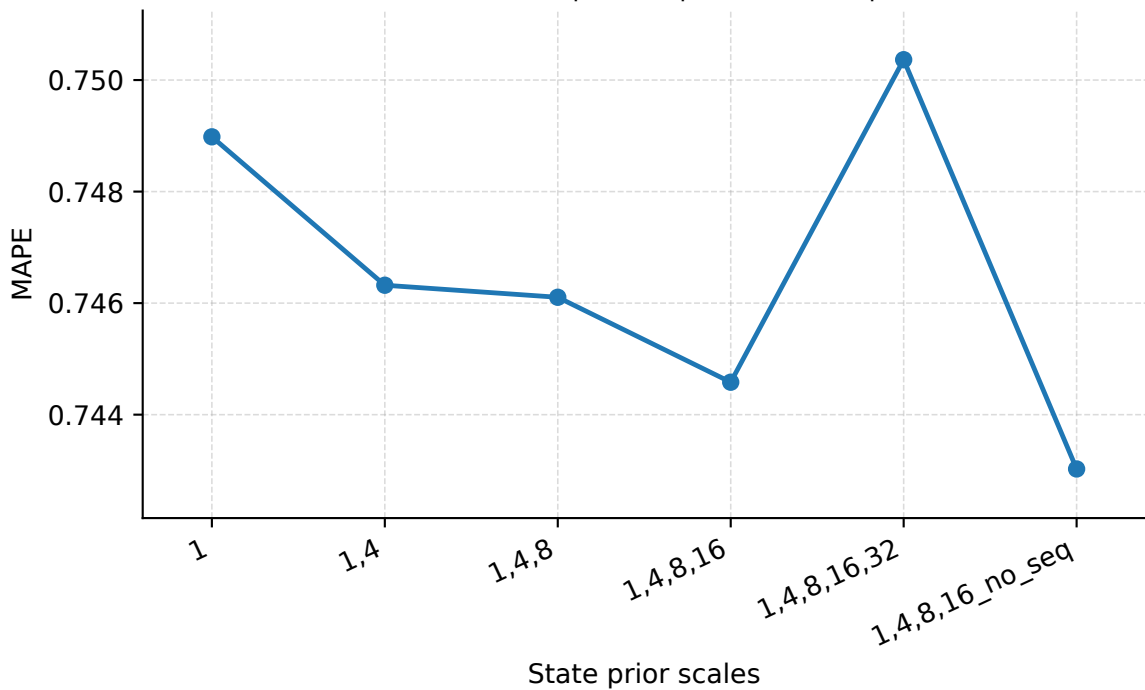
State Prior Scales | Geant | PredLen=20 | MAPE
